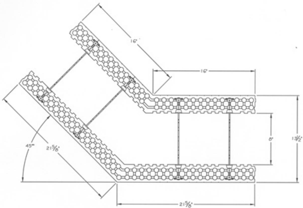
PLAN VIEW
