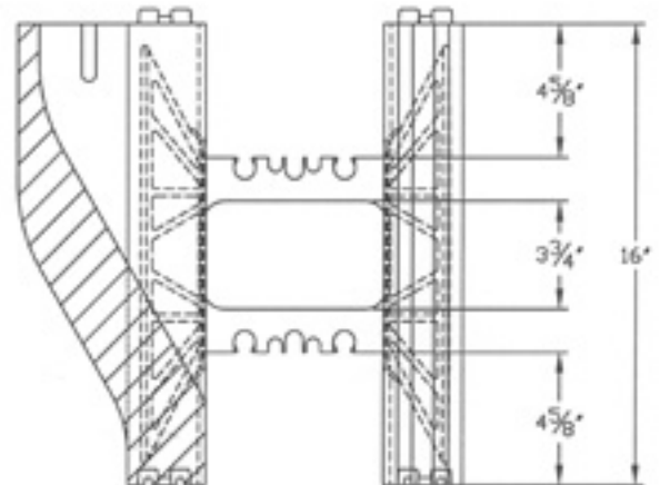
END VIEW
